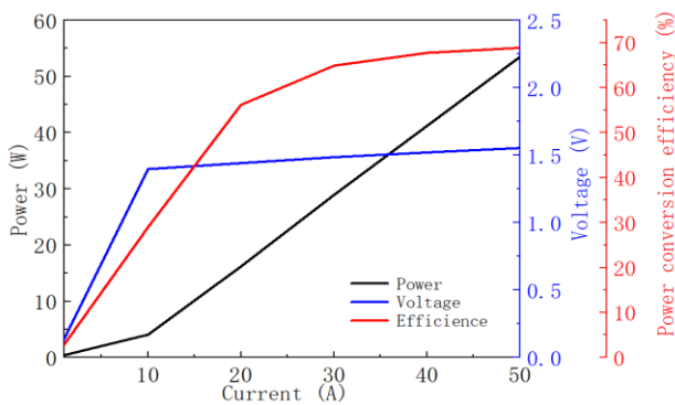
Power-Current-Voltage-Efficiency
